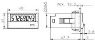
Dimensions CODIX 141 and 143
